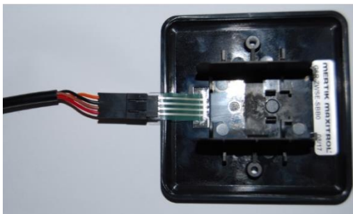
Photo 11 – Wall Switch connection and serial number location
