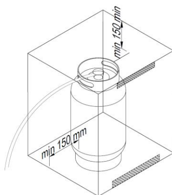
Picture 6 – Housing for gas cylinder
