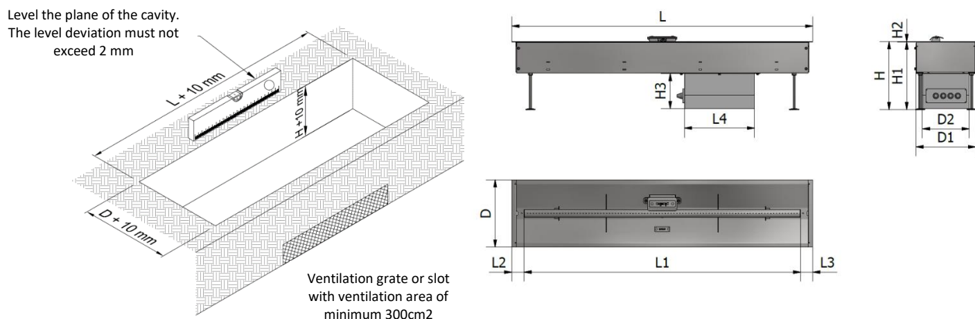
Picture 2 – Cavity measures for units above 1500mm
