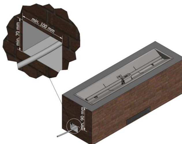
Picture 4 – Installation for LPG type unit
