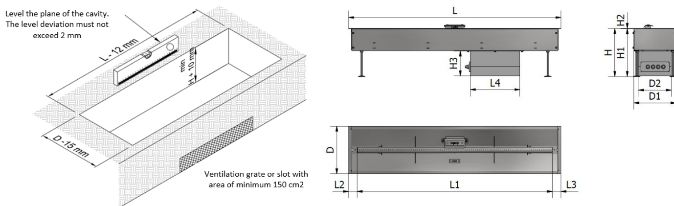
Picture 1 – Cavity measures for units up to 1500mm
