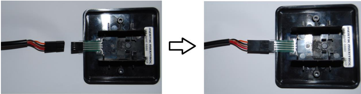
Photo 4 – Wallswitch connection
