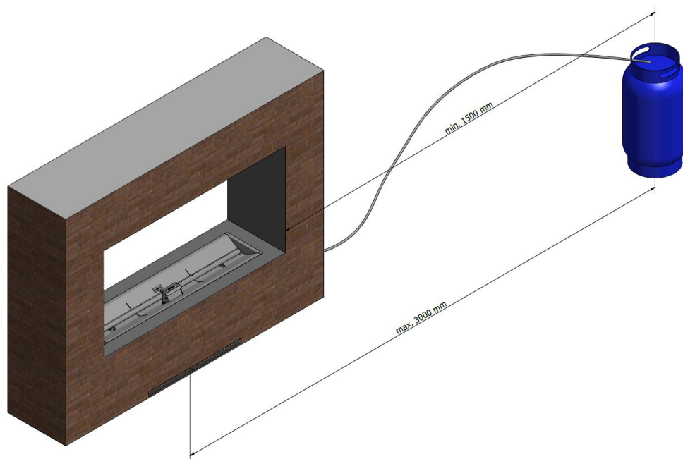
Picture 5 – Location of gas cylinder
